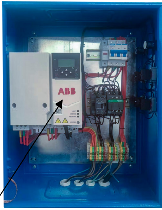
ABB variable-frequency drive
