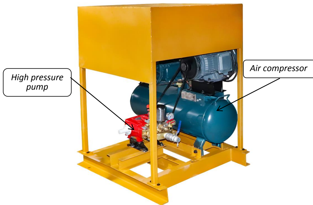
Foam generator
